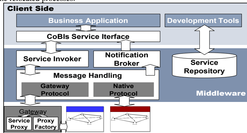
Fig. 3. CoBIs relocated process management architecture
